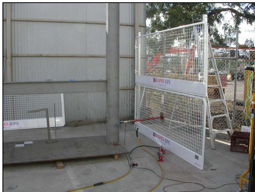
Figure: 4 Subject: Bottom panel outwards horizontal load. .
